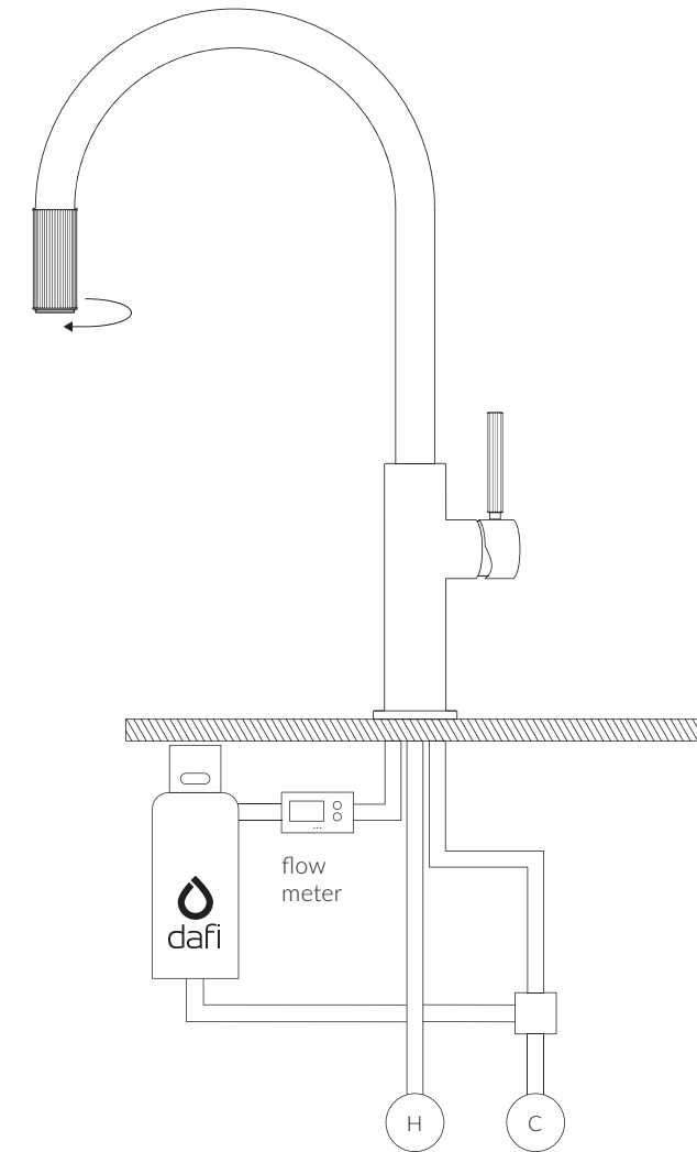
The mixer is available separately or as a set with the water filtration system, equipped with a filter and a precise water flow meter provided by Dafí.
